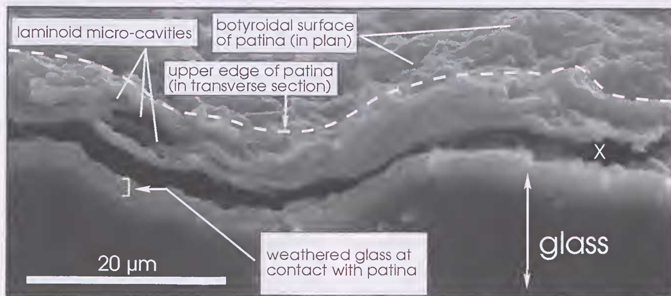
Figure 3. SEM image of a cross-sectional view of patina on glass (sample A1) showing undulating lamination and laminoid micro-cavities. The surface of the patina is botryoidal. The black zone (marked X) between the glass and the patina is a separation crack formed during sample preparation.
